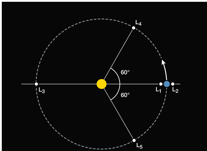
▲ LAGRANGIAN POINTS In a system of two massive bodies orbiting each other (such as the Sun and Earth), five gravitational “balance points” exist where a third, much smaller object can orbit in a constant pattern. A craft at L_2 can always keep the Sun, Earth, and Moon behind itself, making it a frequent choice for space missions. Previous denizens of L_2 include Europe's Planck and Herschel missions; the sky-scanning Gaia spacecraft is currently there.
