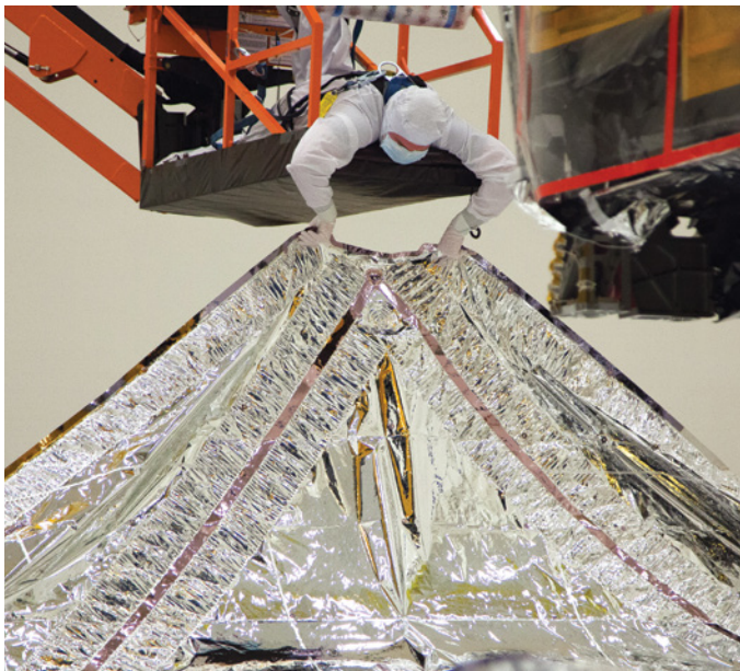
▲ SUNSHIELD Top: This photo from 2014 shows the first time engineers stacked and unfurled a full-size test sunshield. Above: A technician carefully folds the real sunshield in 2020, in preparation for stowing the telescope into its launch configuration.
