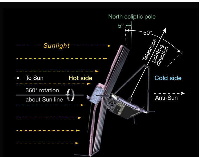
▲ THE VIEW Webb's mirror is perpendicular to its sunshield, and the spacecraft can tilt to point the telescope within a 50° arc while still keeping the mirror and instruments safely in shadow. It can also rotate full circle. Over time, Webb will see the entire sky as it orbits the Sun.
