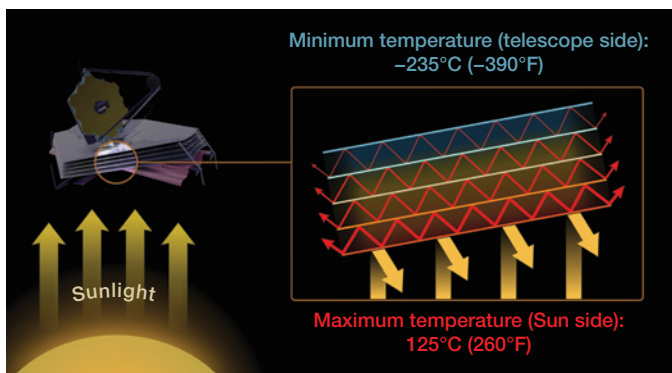
▲ PARASOL The five-layer design of Webb's sunshield protects its mirror and instruments from unwanted infrared radiation from the Sun, Earth, and Moon. Because none of the layers touch, heat doesn't conduct from one layer to another and instead flows to the layers' edges and into space.
