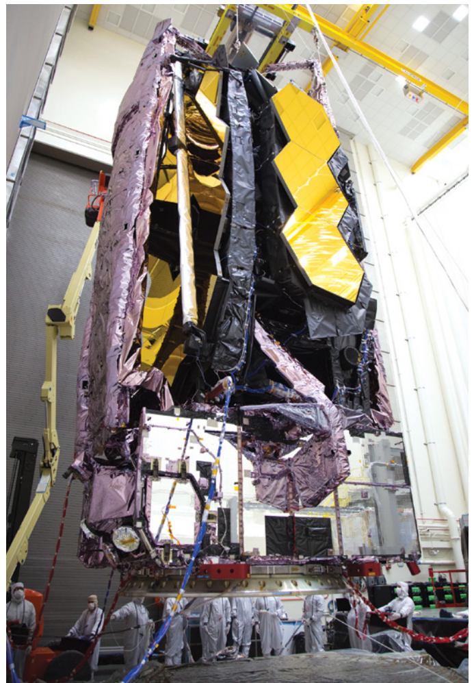
▼ FOLDED FOR LAUNCH TEST The telescope successfully endured deafening noise and jarring vibrations tuned to simulate conditions aboard the Ariane 5 rocket during launch. These 2020 tests were the last environmental tests before launch.
