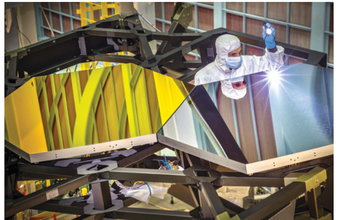
▲ GO FOR GOLD An optical engineer examines two test mirror segments, one coated in gold. The frame is a composite material designed to handle Webb's space environment.
