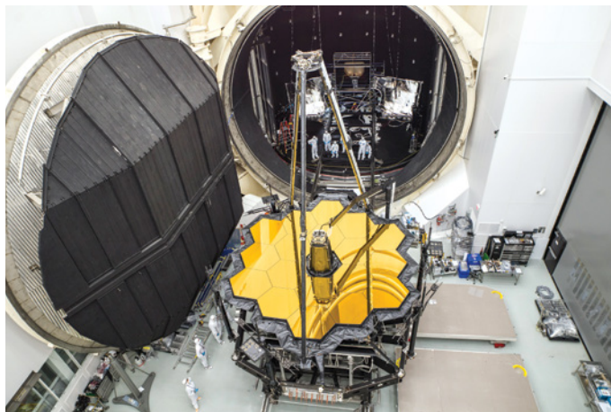
▲ CHAMBER A Webb emerges from months of cryogenic vacuum testing in 2017.
