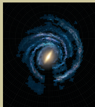
Artist's concept of our Milky Way map under construction
